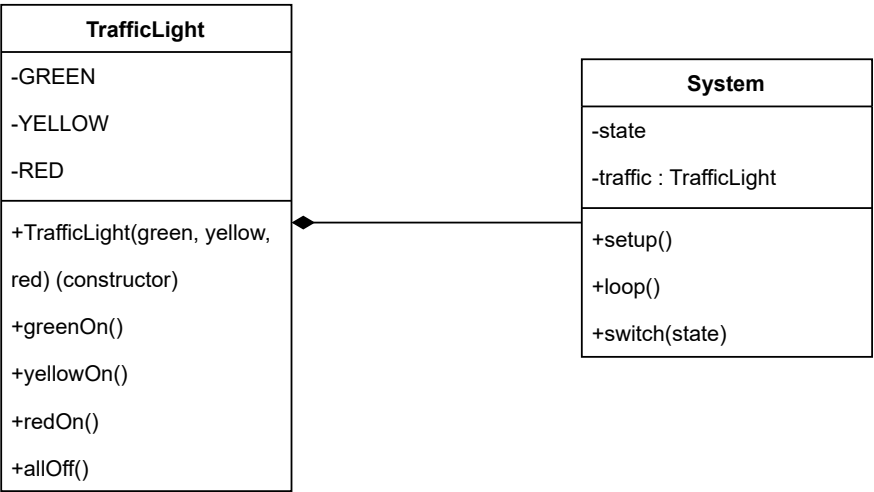
Class Diagram for Traffic light system
